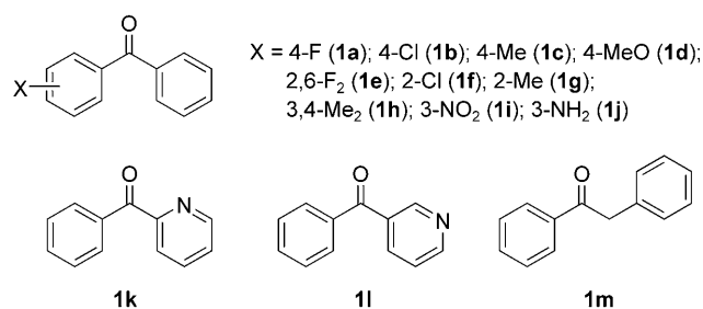
Figure 1. Substituted benzophenones, benzoylpyridines, and benzyl phenyl ketone.
