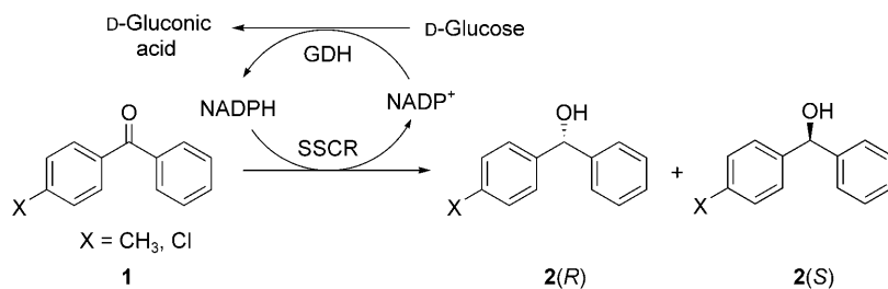
Scheme 1. SSCR-catalyzed reduction of diaryl ketones with a glucose dehydrogenase/D-glucose NADPH regeneration system.
